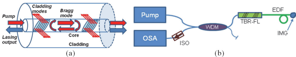
Fig. 6.4. (a) Structure of the TBR-FL, and (b) experimental setup. OSA = optical spectrum analyser, WDM = wavelength division multiplexer, EDF = erbium-doped fibre, ISO = isolator, IMG = index matching gel.
