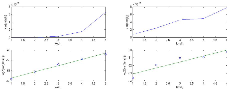
Fig. 8. Variances of details plotted as a function of the decomposition level j for two processes: a) I_0 (slope \beta = 3.0092 ) and b) I_2 (slope \beta = 0.7700 ) (Planinšič & Petek, 2008).
