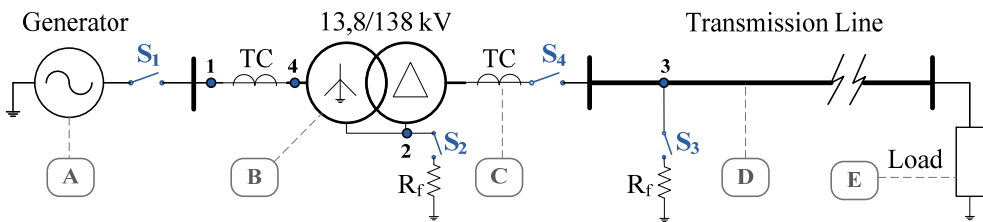
Fig. 6. Simulated electric power system.
