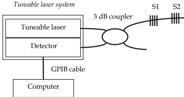
Fig. 4.2. Experimental setup of the multiplexed AMCFBG system.
