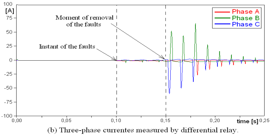
Fig. 9. External faults removal simulation.
