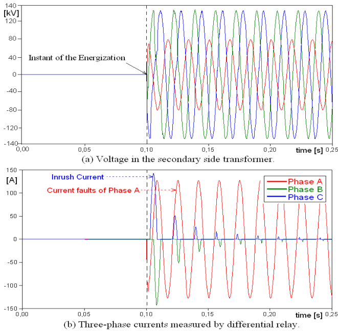
Fig. 8. Energization and internal faults simulation on PT.
