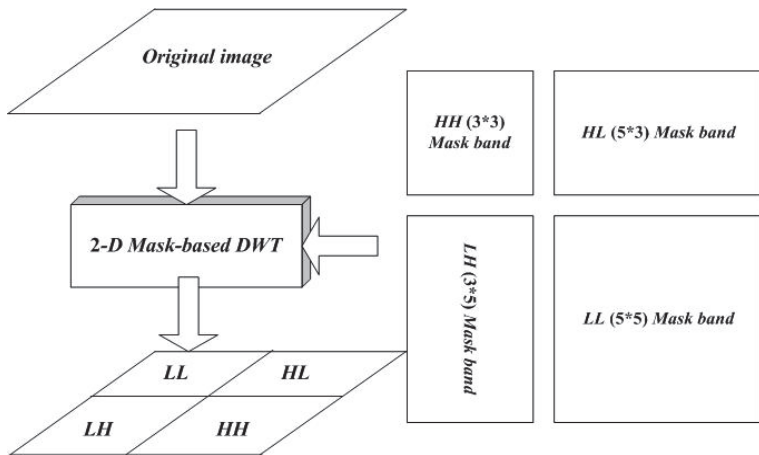
Fig. 5. The system block diagram of 2-D SMDWT.
