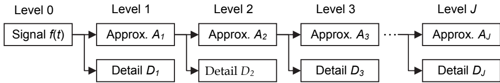
Fig. 2.1. Multistage decomposition of a signal using QMFB.
