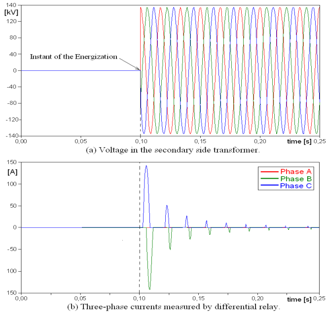
Fig. 7. Energization simulation on PT.
