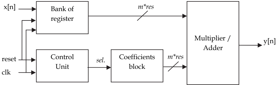
Fig. 12. Architecture of Discrete Wavelet Transform.
