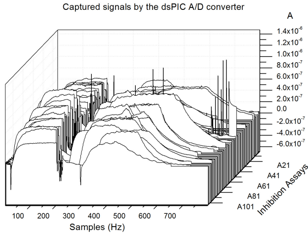
Fig. 7. The matrix of the voltammograms captured by the ADC of dsPIC30F6014.
