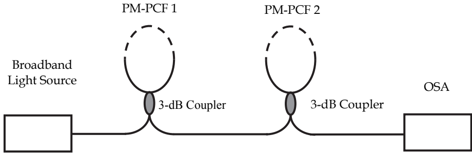
Fig. 5.1. Experimental setup of in series multiplexing technique for PM-PCF based Sagnac interferometric sensor.
