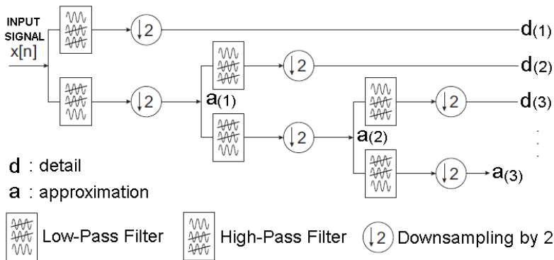
Fig. 2. DWT filter bank framework.
