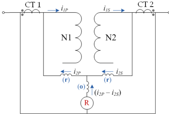
Fig. 3. Differential relay connections.
