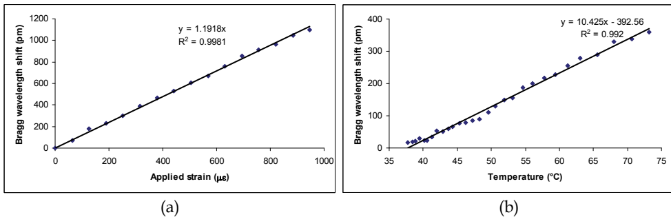
Fig. 3.5. (a) Strain and (b) temperature responses of the FBG sensor.
