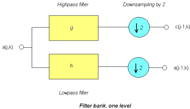
Fig. 5. One stage of analysis filter bank
