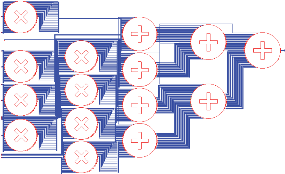
Fig. 13. RTL: Multiplier/Adder block.
